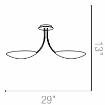
50152 Krome Reflected Up Light Semi-Flush Lamping 2Lt x 150w Halogen 120v J118 (T-3 Base) Finish CH CETL Damp
