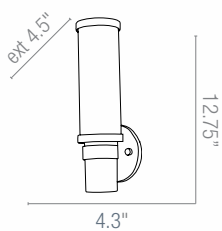
50569 Zylinder Wall Fixture
